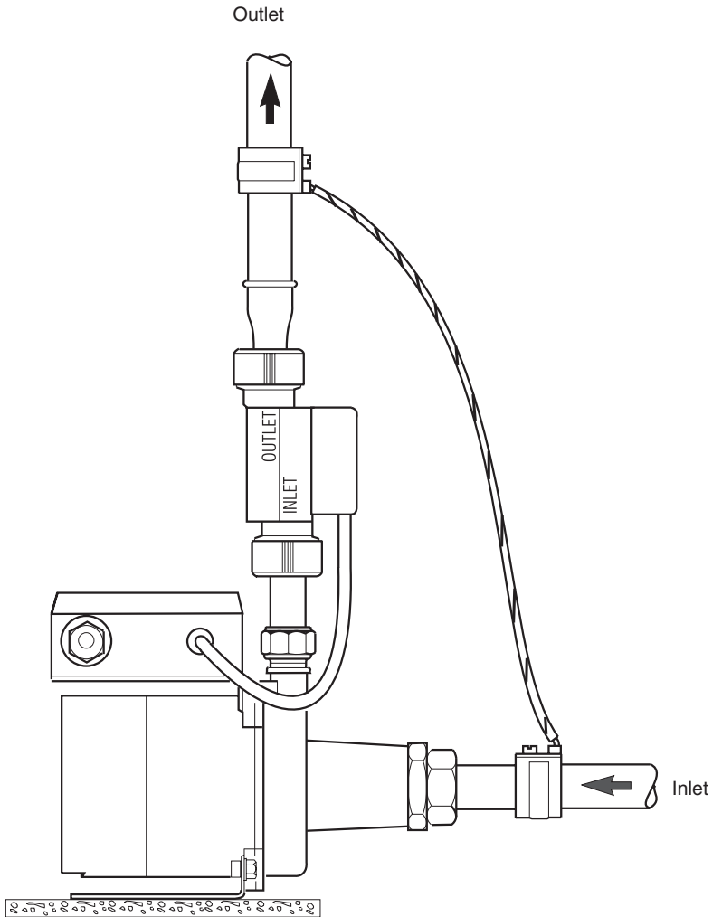
Pipe Bonding Details Figure 7
